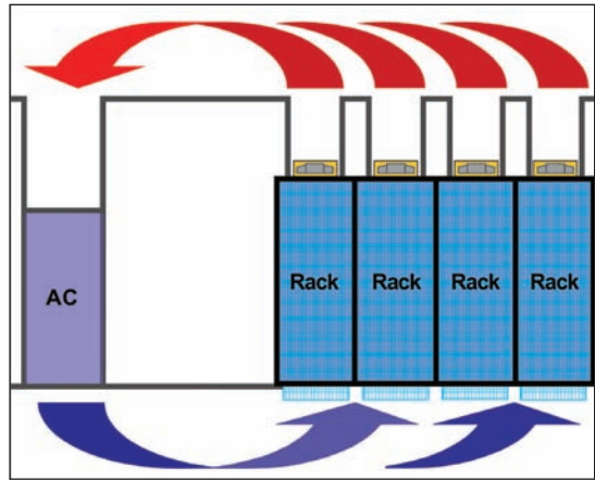
Figure 5: High-density heat containment system.
