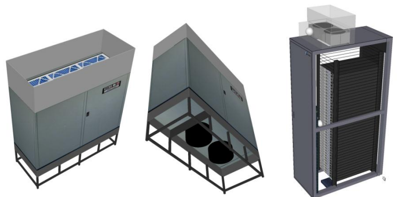
26 Ton Cooling Unit with Return Duct Extension and Sub-floor Plug Fans
