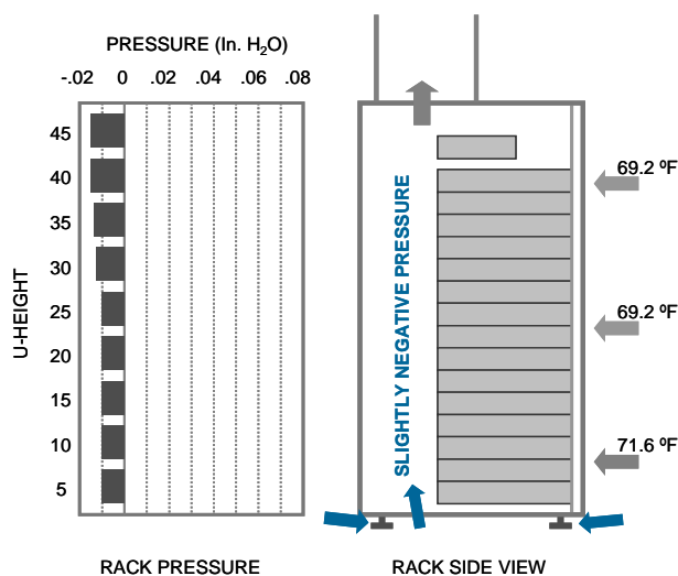
Figure 4: Active rack fan releasing 1640 CFM to ceiling plenum for 1400 CFM load represents 240 CFM (17%) cool air bypass.
