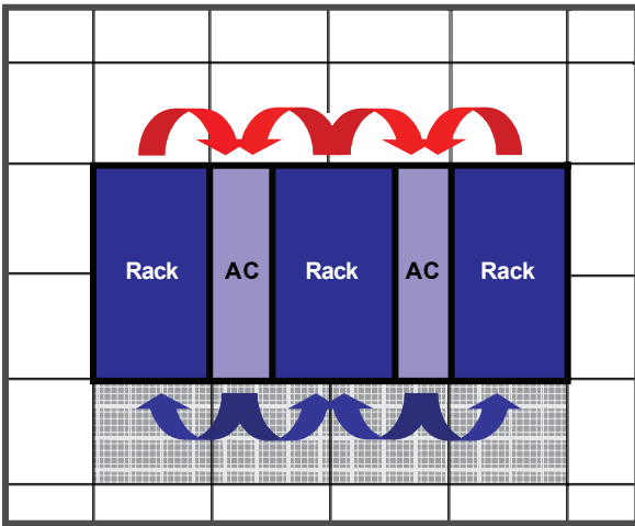
Airflow distribution patterns with cooling units placed in the row - view looking at top of cabinet row.
