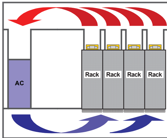
Airflow distribution patterns with HDHC method of cooling - view looking at front of cabinet row.
