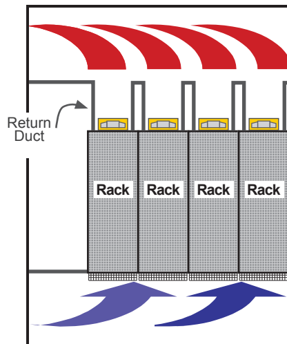
Return duct exhaust within a heat containment distribution system.
