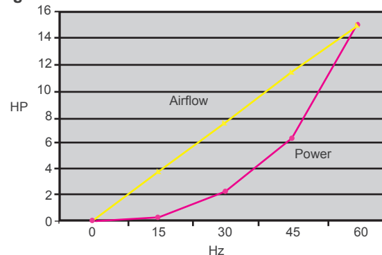
Cubic fan laws demonstrate significant power savings at slightly reduce airflow rates.
