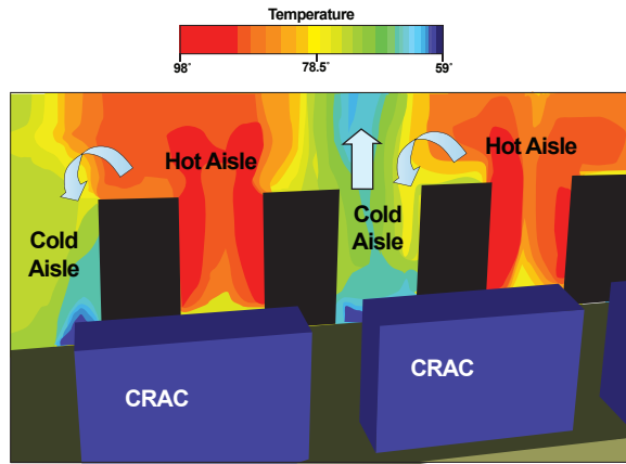
Rack inlet temperature is 76 Deg F with conventional cooling and 50% excess cool air supply.
