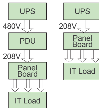
Two typical power flow diagrams for UPS to the IT equipment load.
