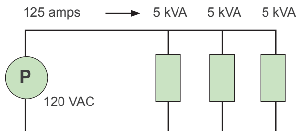
Amperage in a single-phase circuit
