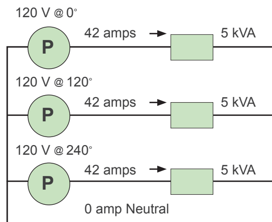
Amperage in a three-phase circuit
