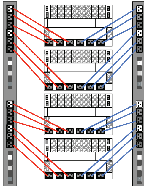
Power distributed to four HP C-class chassis.
