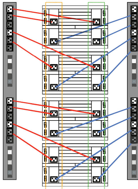
Power distributed to an IBM BladeCenter chassis
